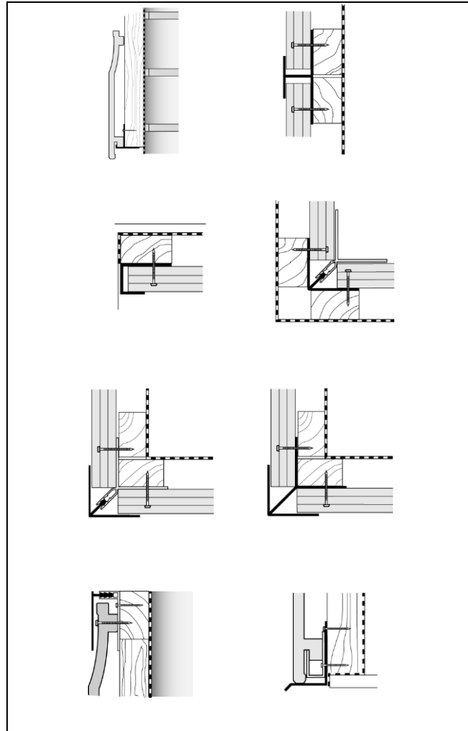
Figure 3 Typical installation details
